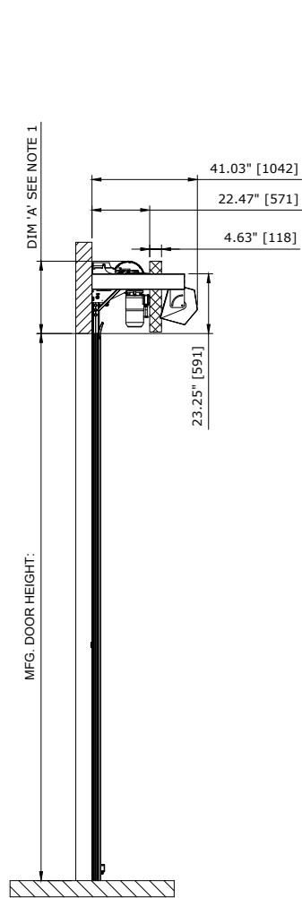
LEFT VIEW
