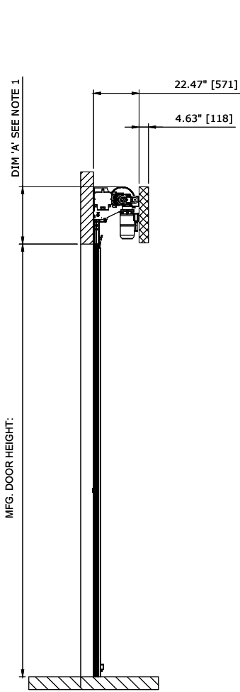
LEFT VIEW
