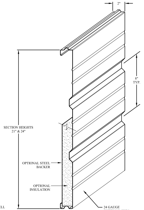
ISOMETRIC PROFILE
