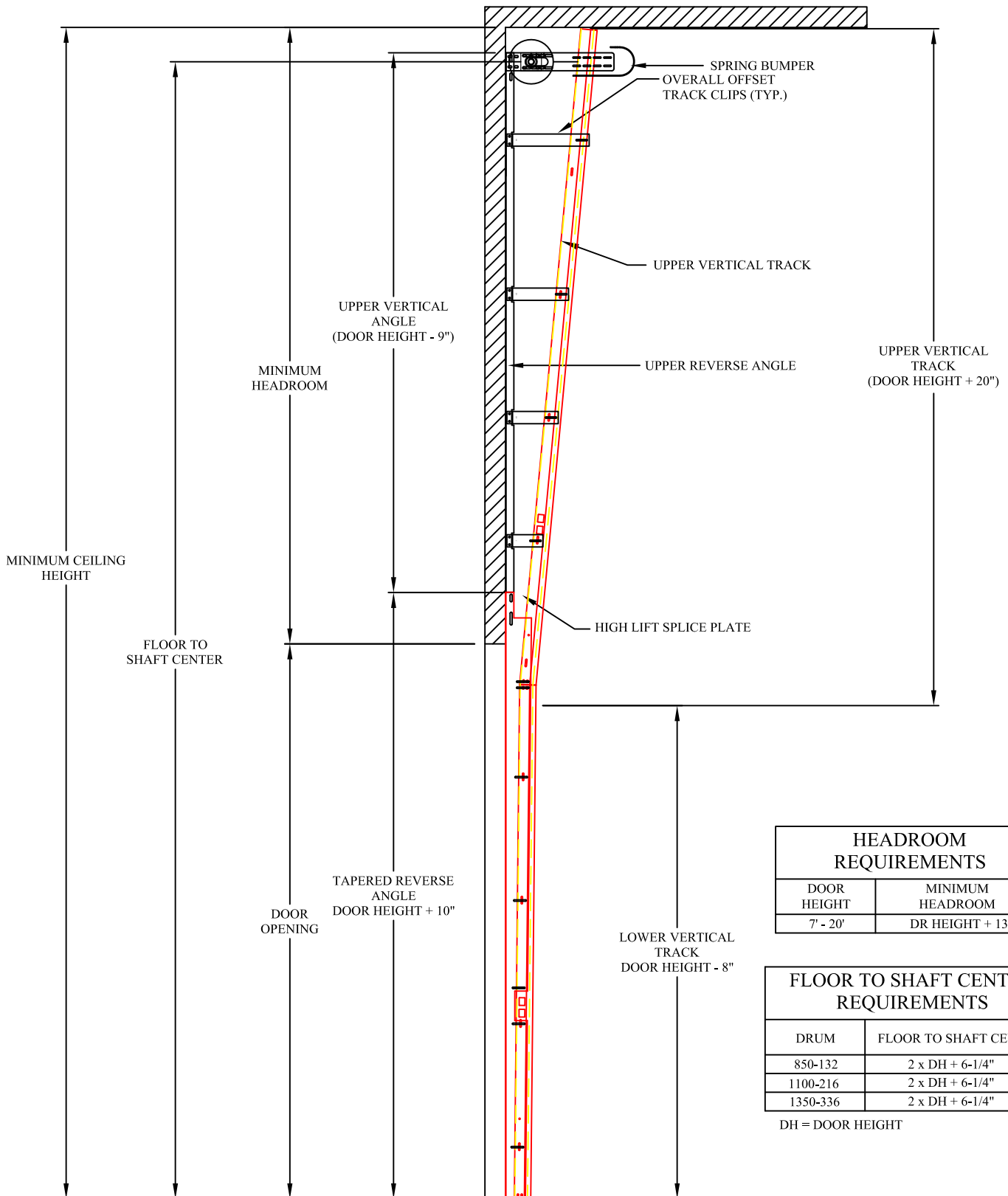
VERTICAL LIFT STANDARD 3" TAPERED REVERSE ANGLE MOUNT TRACK SET DETAIL
