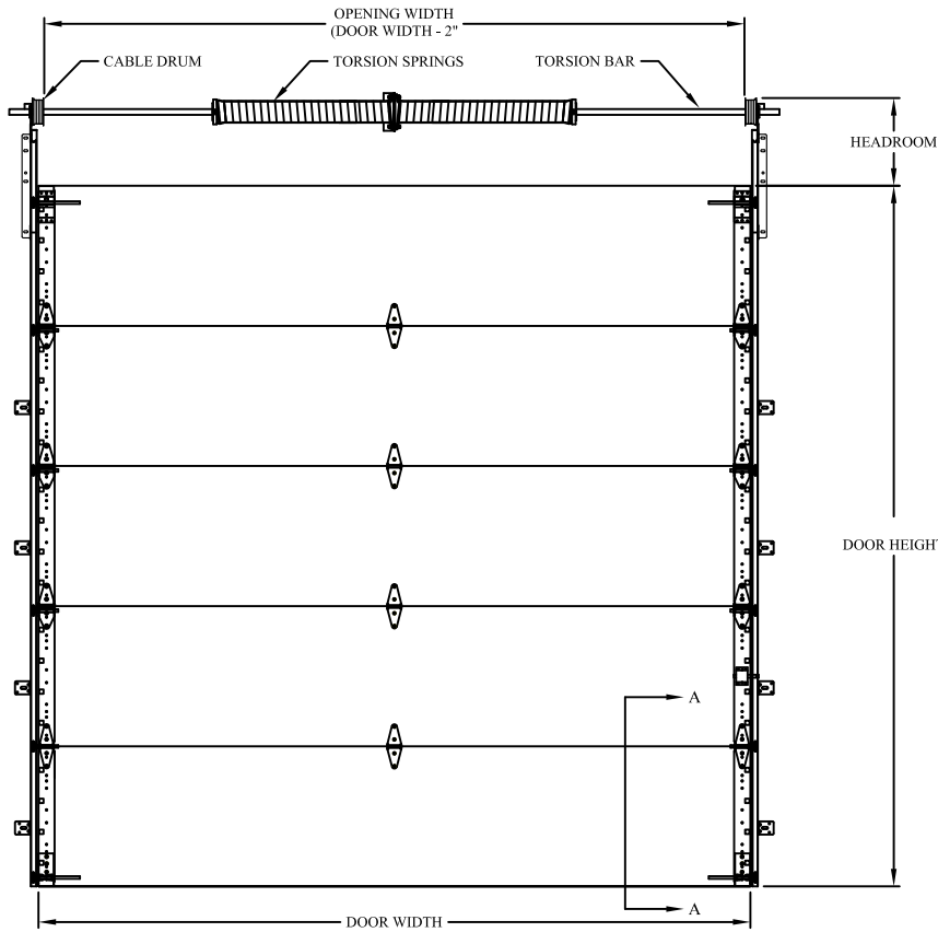
INTERIOR ELEVATION
